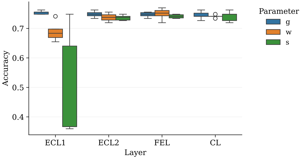
Parameter Performance by Layer
